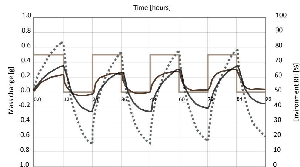
Mass change of plasters when exposed to changing relative humidity
